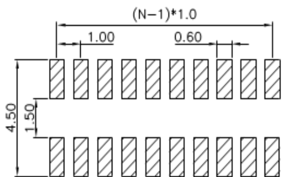
RECOMMEND PCB LAYOUT(TOLERANCE ±0.05)
