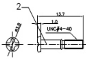
Short BOLT
