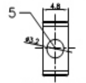
SMALL WASHER
