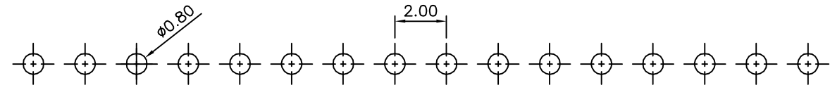
Recommended P.C.B. Layout
